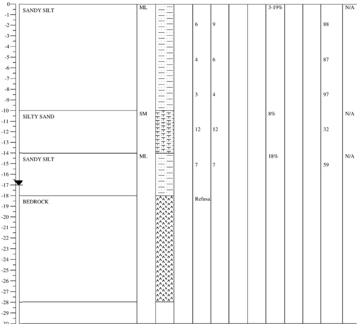
Figure 4.6 Boring B4 performed by DICTUC [2012]; from Gebhart [2016].
