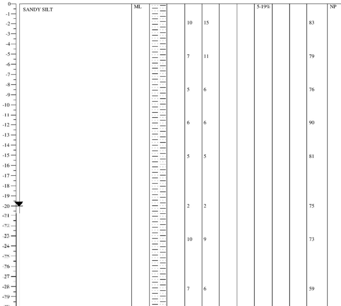
Figure 4.5 Boring B3 performed by DICTUC [2012]; from Gebhart [2016].
