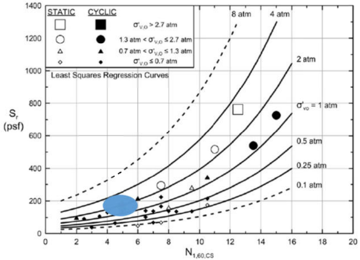
Figure 7.11 Las Palmas data point with respect to Weber et al. [2015].
