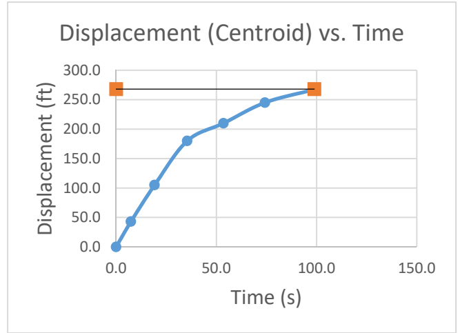
Figure 6.5 Example trial of incremental momentum method (IMM) after Weber [2015].
